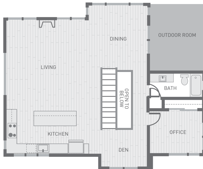
3RD FLOOR
